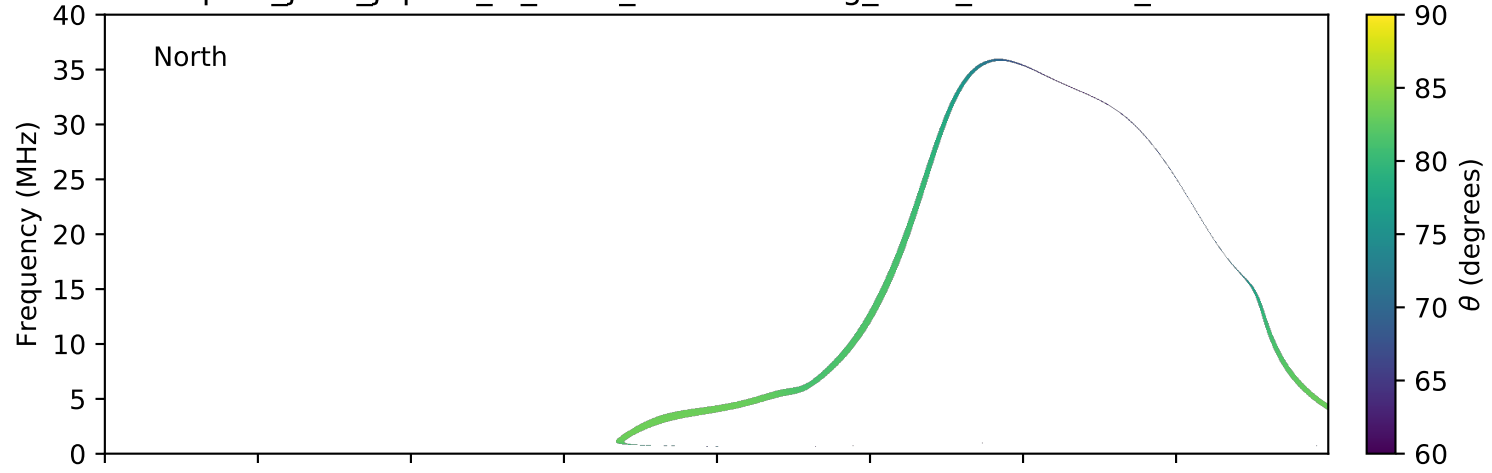
expres_juno_jupiter_io_isaac_lossc-wid1deg_3kev_20170206_v01.cdf
