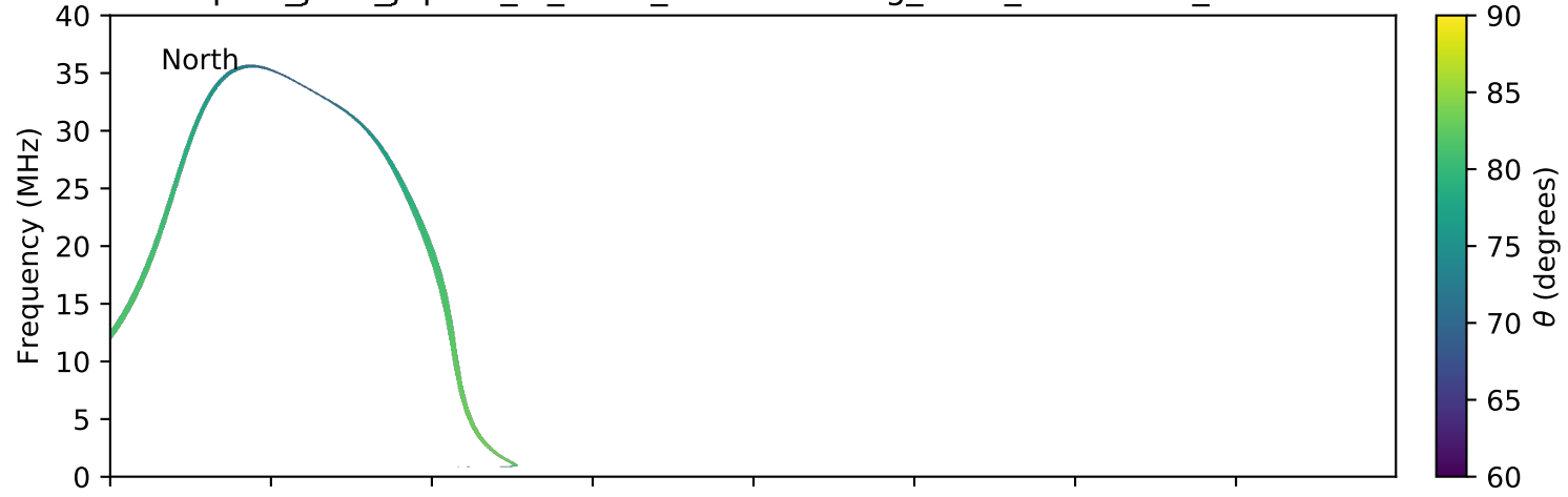
expres_juno_jupiter_io_isaac_lossc-wid1deg_3kev_20170205_v01.cdf
