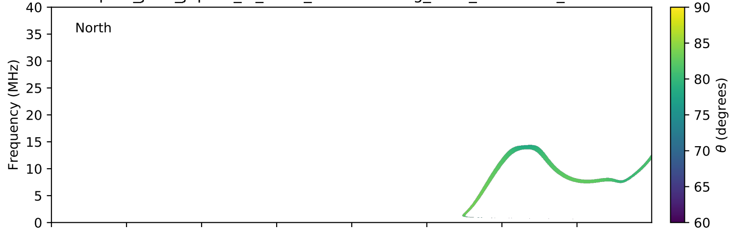
expres_juno_jupiter_io_isaac_lossc-wid1deg_3kev_20170204_v01.cdf
