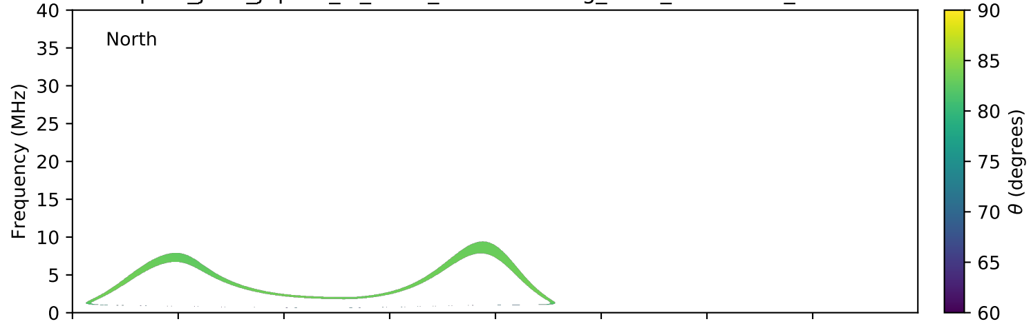
expres_juno_jupiter_io_isaac_lossc-wid1deg_3kev_20170203_v01.cdf
