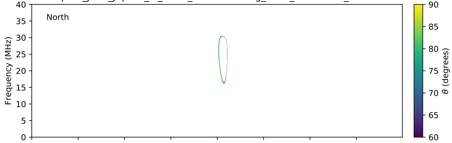
expres_juno_jupiter_io_isaac_lossc-wid1deg_3kev_20170202_v01.cdf
