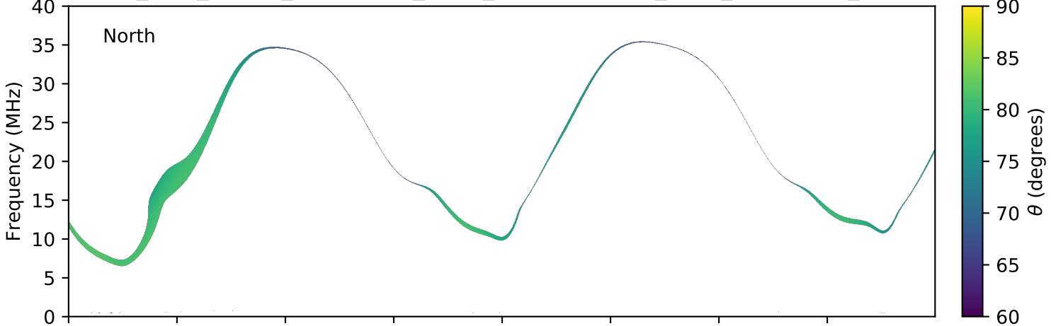
expres_juno_jupiter_ganymede_isaac_lossc-wid1deg_3kev_20170228_v01.cdf
