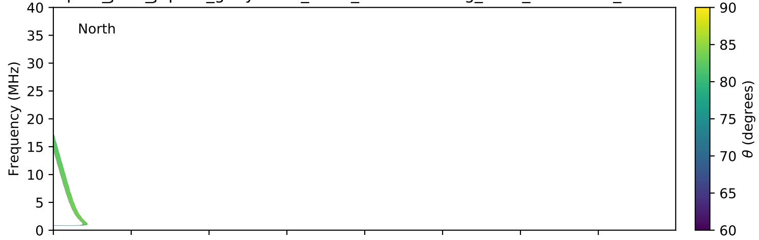
expres_juno_jupiter_ganymede_isaac_lossc-wid1deg_3kev_20170223_v01.cdf
