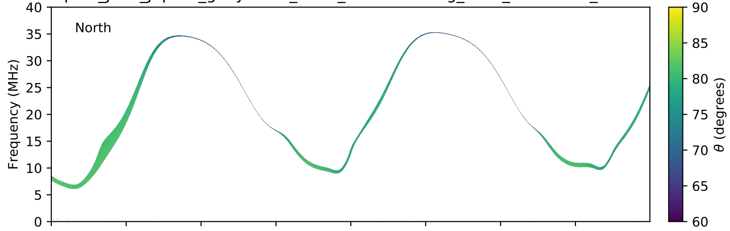
expres_juno_jupiter_ganymede_isaac_lossc-wid1deg_3kev_20170221_v01.cdf
