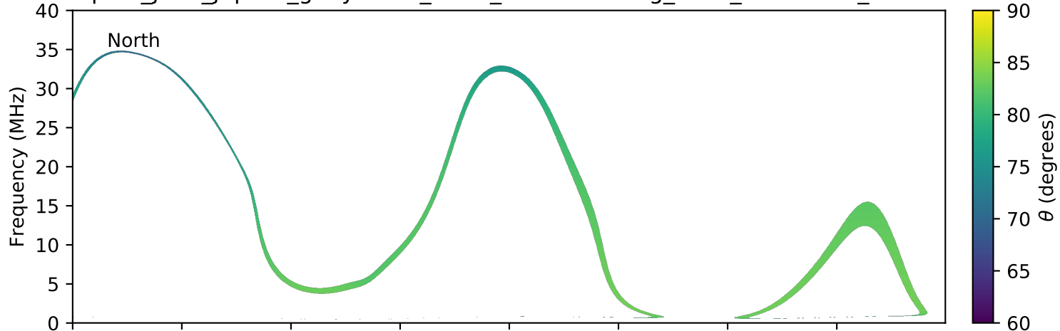
expres_juno_jupiter_ganymede_isaac_lossc-wid1deg_3kev_20170215_v01.cdf
