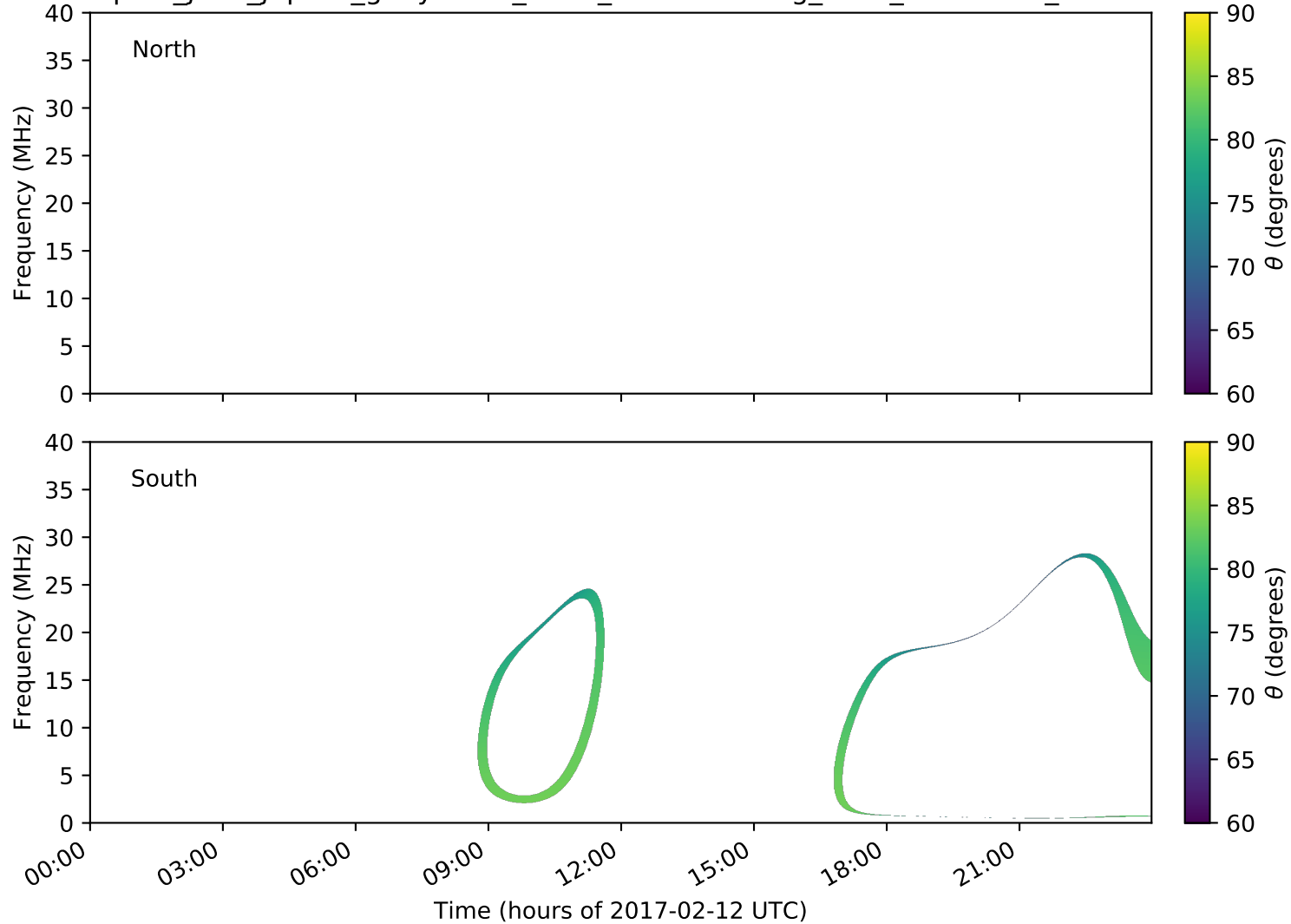
expres_juno_jupiter_ganymede_isaac_lossc-wid1deg_3kev_20170212_v01.cdf
