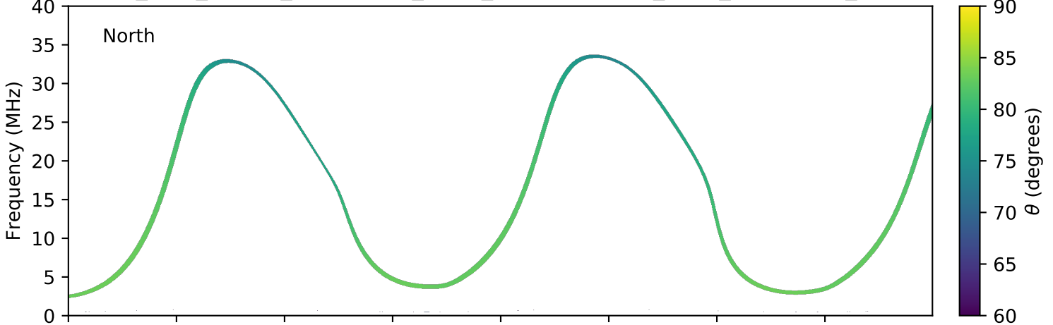
expres_juno_jupiter_ganymede_isaac_lossc-wid1deg_3kev_20170207_v01.cdf
