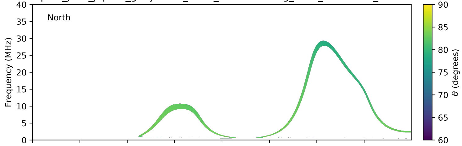
expres_juno_jupiter_ganymede_isaac_lossc-wid1deg_3kev_20170206_v01.cdf
