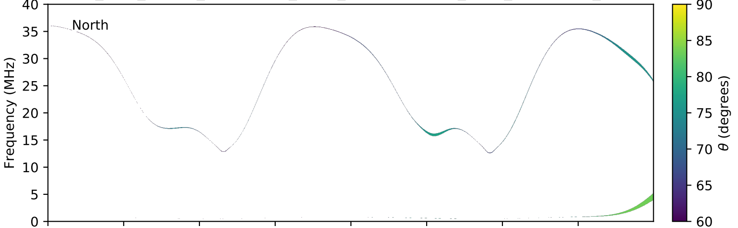
expres_juno_jupiter_ganymede_isaac_lossc-wid1deg_3kev_20170201_v01.cdf
