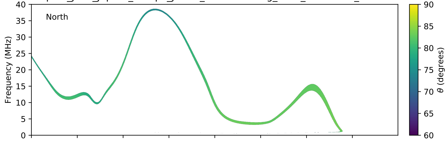
expres_juno_jupiter_europa_jrm09_lossc-wid1deg_3kev_20170211_v01.cdf
