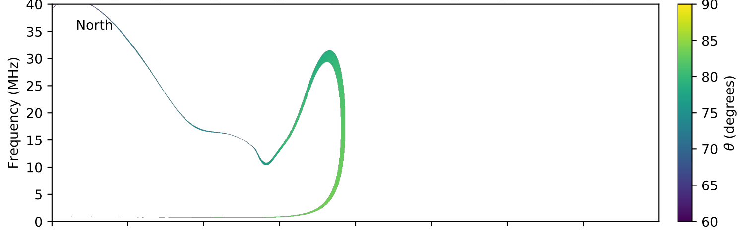
expres_juno_jupiter_europa_jrm09_lossc-wid1deg_3kev_20170201_v01.cdf
