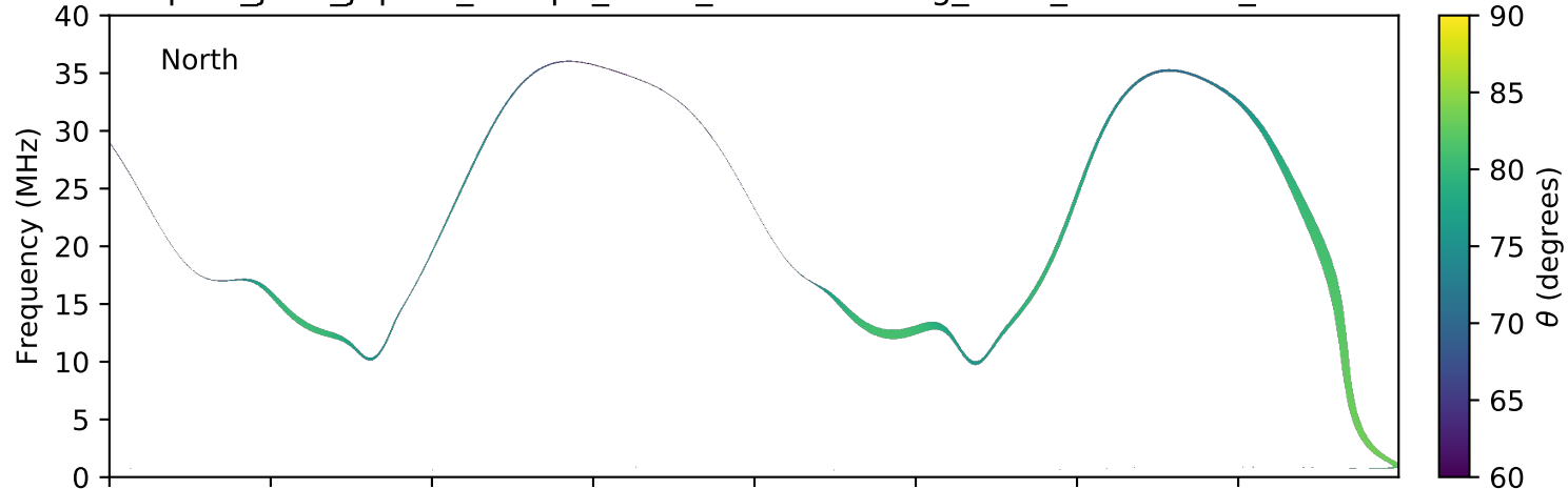
expres_juno_jupiter_europa_isaac_lossc-wid1deg_3kev_20170225_v01.cdf
