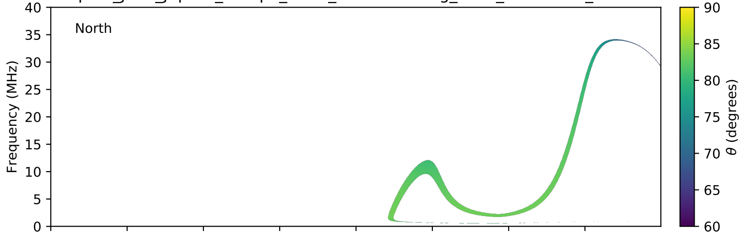
expres_juno_jupiter_europa_isaac_lossc-wid1deg_3kev_20170224_v01.cdf
