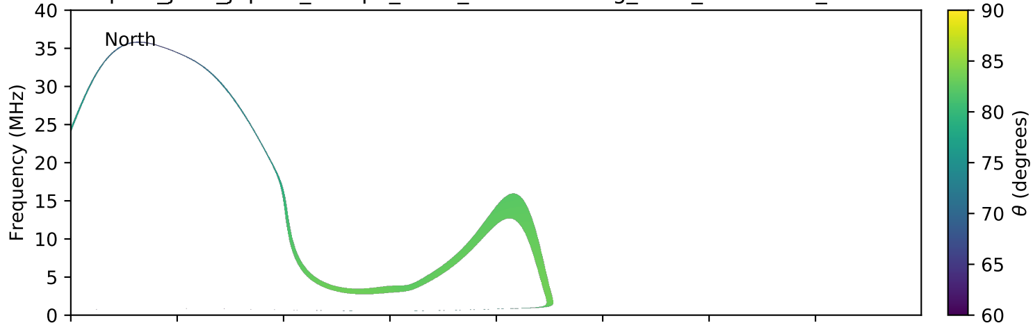
expres_juno_jupiter_europa_isaac_lossc-wid1deg_3kev_20170222_v01.cdf
