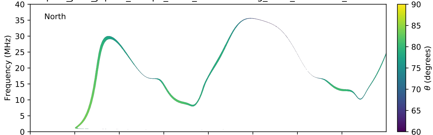
expres_juno_jupiter_europa_isaac_lossc-wid1deg_3kev_20170221_v01.cdf
