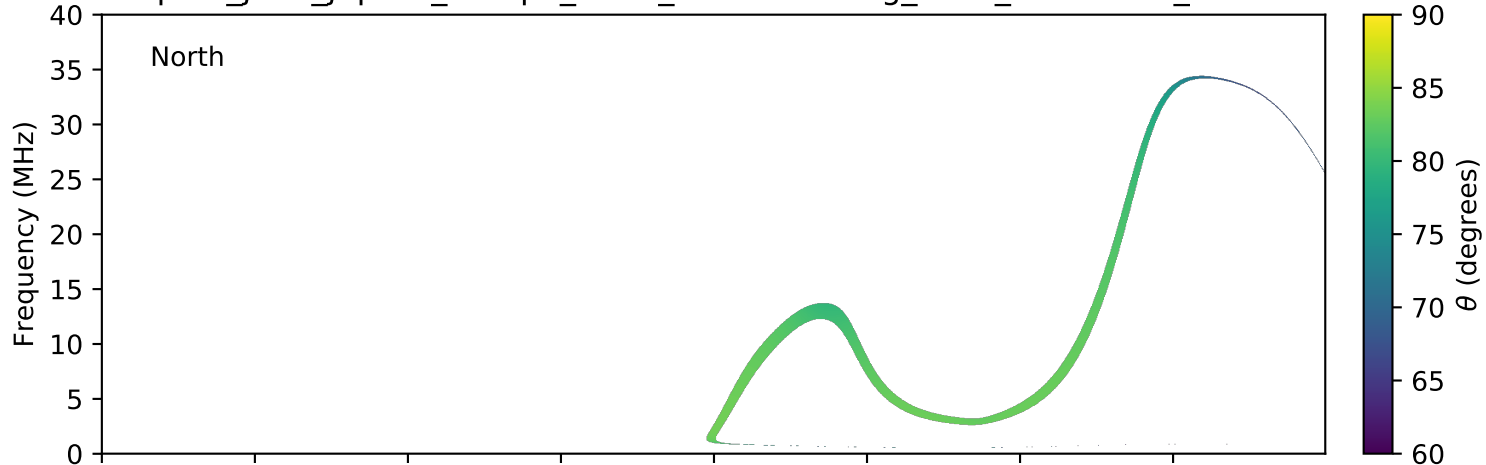
expres_juno_jupiter_europa_isaac_lossc-wid1deg_3kev_20170217_v01.cdf
