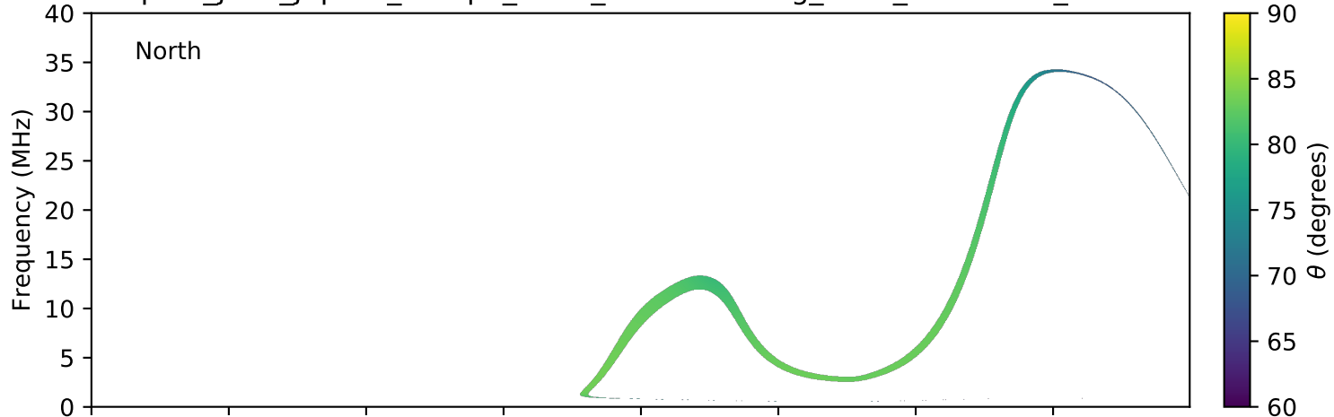
expres_juno_jupiter_europa_isaac_lossc-wid1deg_3kev_20170210_v01.cdf
