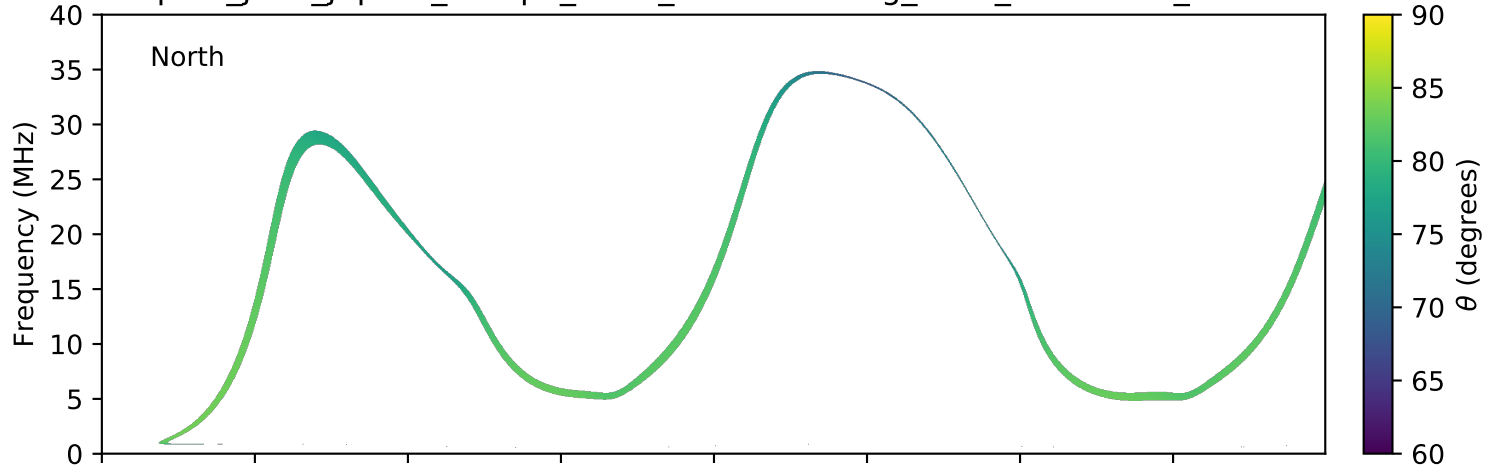
expres_juno_jupiter_europa_isaac_lossc-wid1deg_3kev_20170207_v01.cdf
