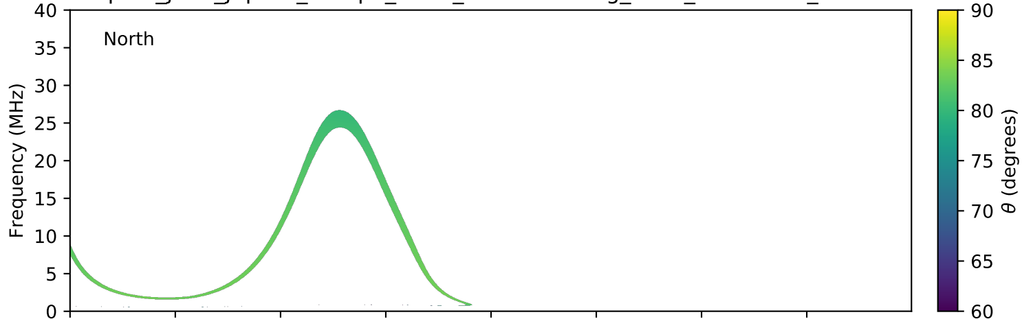
expres_juno_jupiter_europa_isaac_lossc-wid1deg_3kev_20170204_v01.cdf
