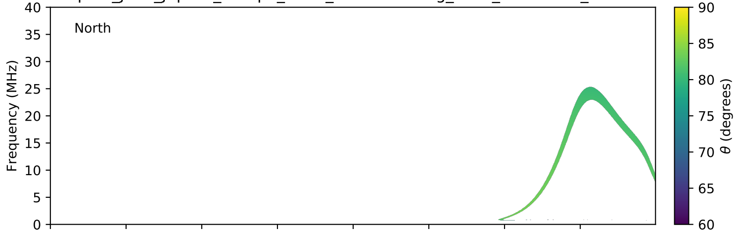
expres_juno_jupiter_europa_isaac_lossc-wid1deg_3kev_20170203_v01.cdf
