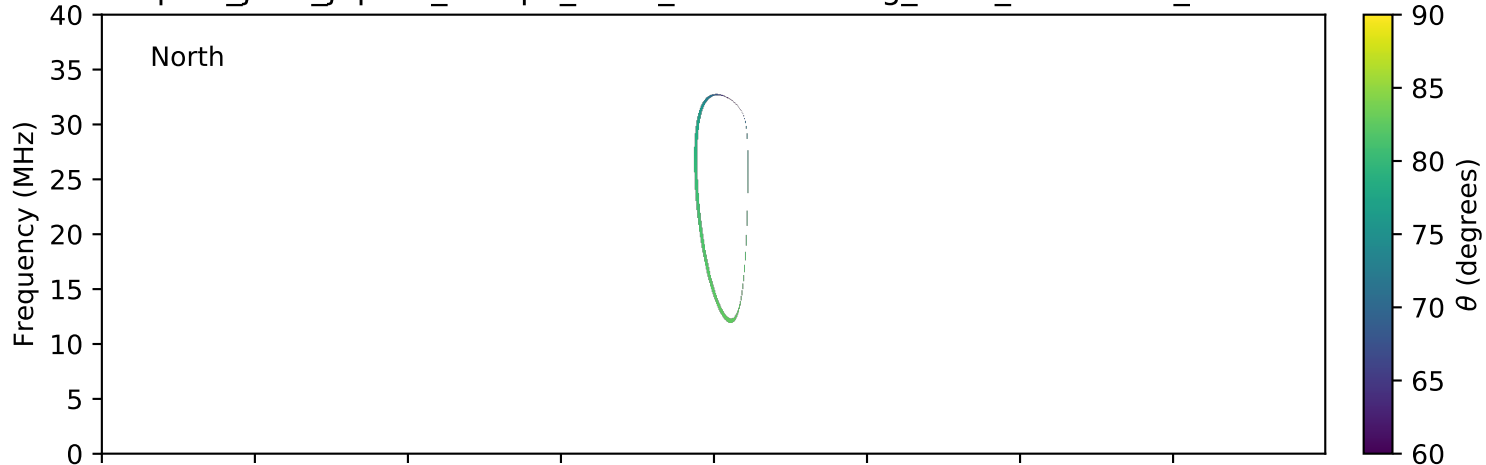
expres_juno_jupiter_europa_isaac_lossc-wid1deg_3kev_20170202_v01.cdf
