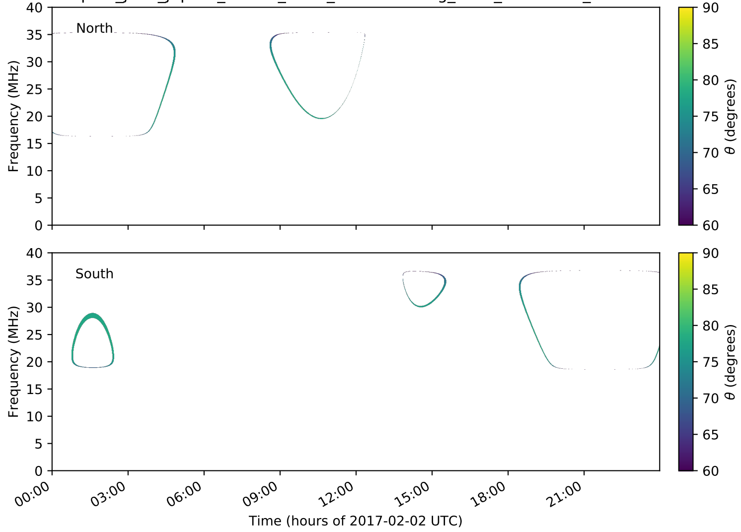
expres_juno_jupiter_50d-0r_isaac_lossc-wid1deg_9kev_20170202_v01.cdf
