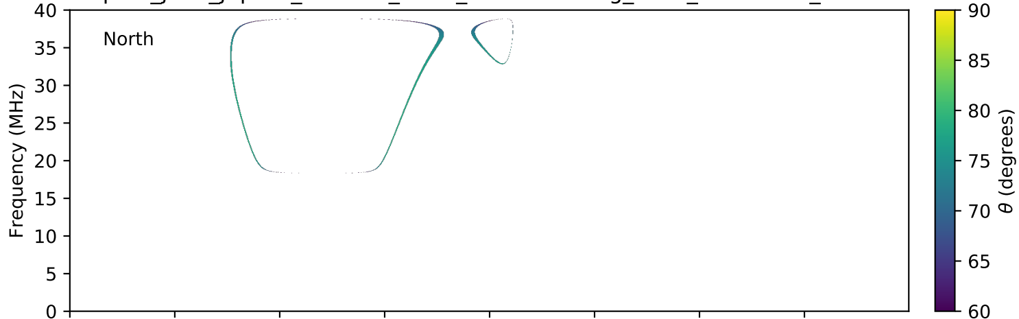
expres_juno_jupiter_255d-0r_isaac_lossc-wid1deg_9kev_20170202_v01.cdf
