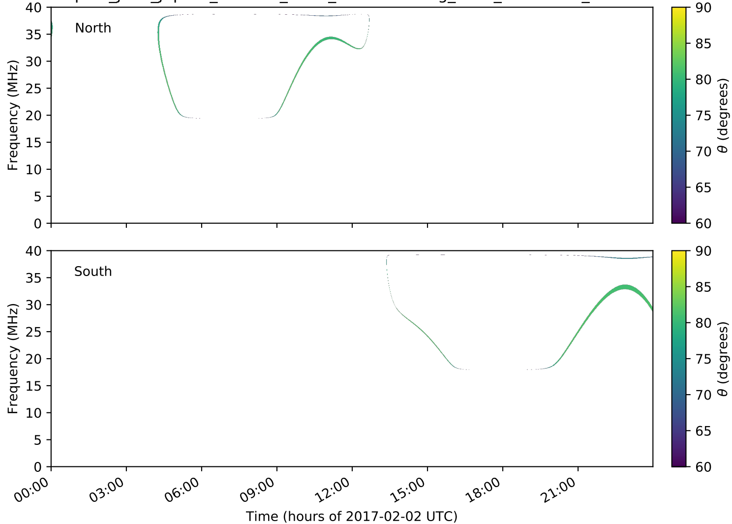
expres_juno_jupiter_253d-0r_isaac_lossc-wid1deg_5kev_20170202_v01.cdf
