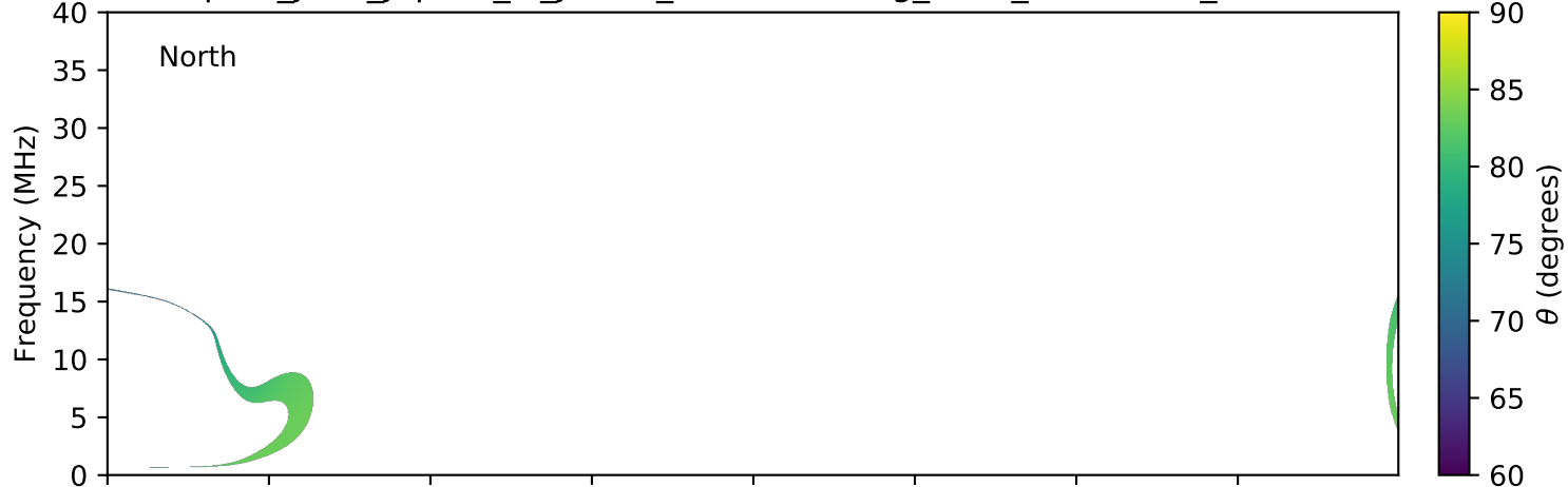
expres_juno_jupiter_io_jrm09_lossc-wid1deg_3kev_20170131_v01.cdf
