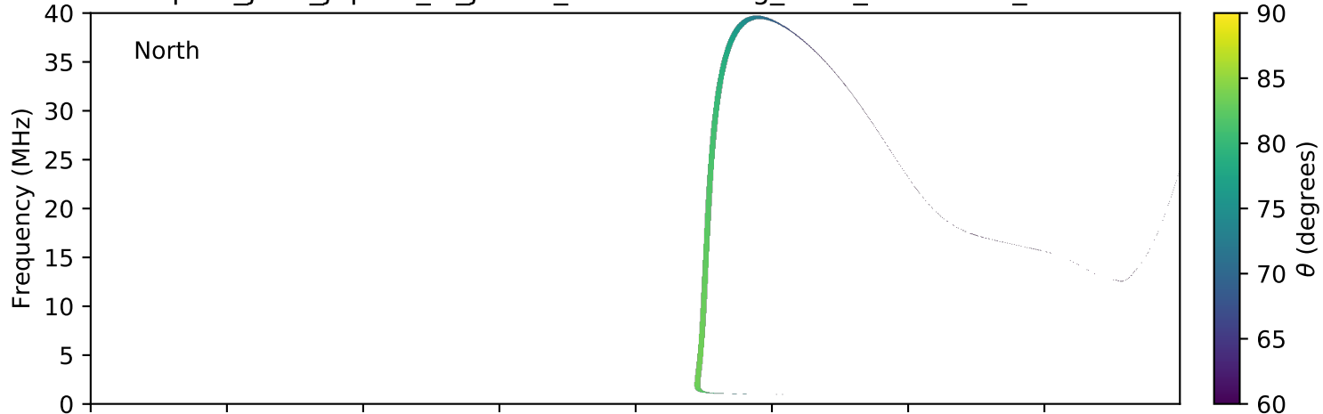
expres_juno_jupiter_io_jrm09_lossc-wid1deg_3kev_20170128_v01.cdf
