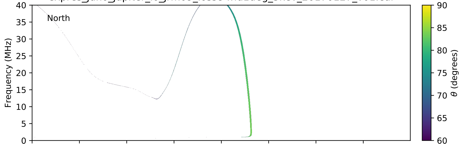
expres_juno_jupiter_io_jrm09_lossc-wid1deg_3kev_20170127_v01.cdf
