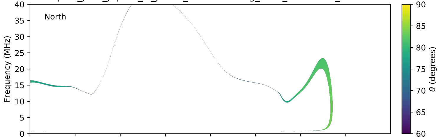
expres_juno_jupiter_io_jrm09_lossc-wid1deg_3kev_20170125_v01.cdf
