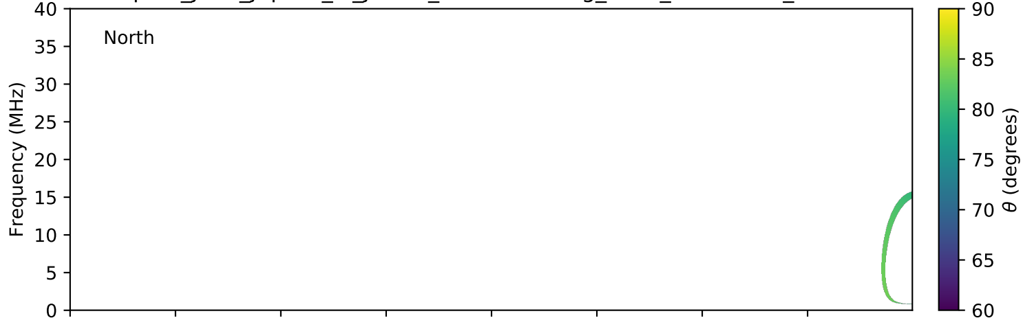
expres_juno_jupiter_io_jrm09_lossc-wid1deg_3kev_20170124_v01.cdf
