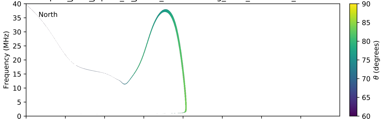
expres_juno_jupiter_io_jrm09_lossc-wid1deg_3kev_20170120_v01.cdf
