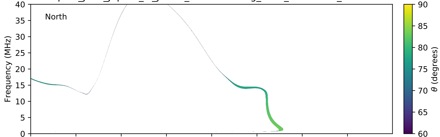
expres_juno_jupiter_io_jrm09_lossc-wid1deg_3kev_20170118_v01.cdf
