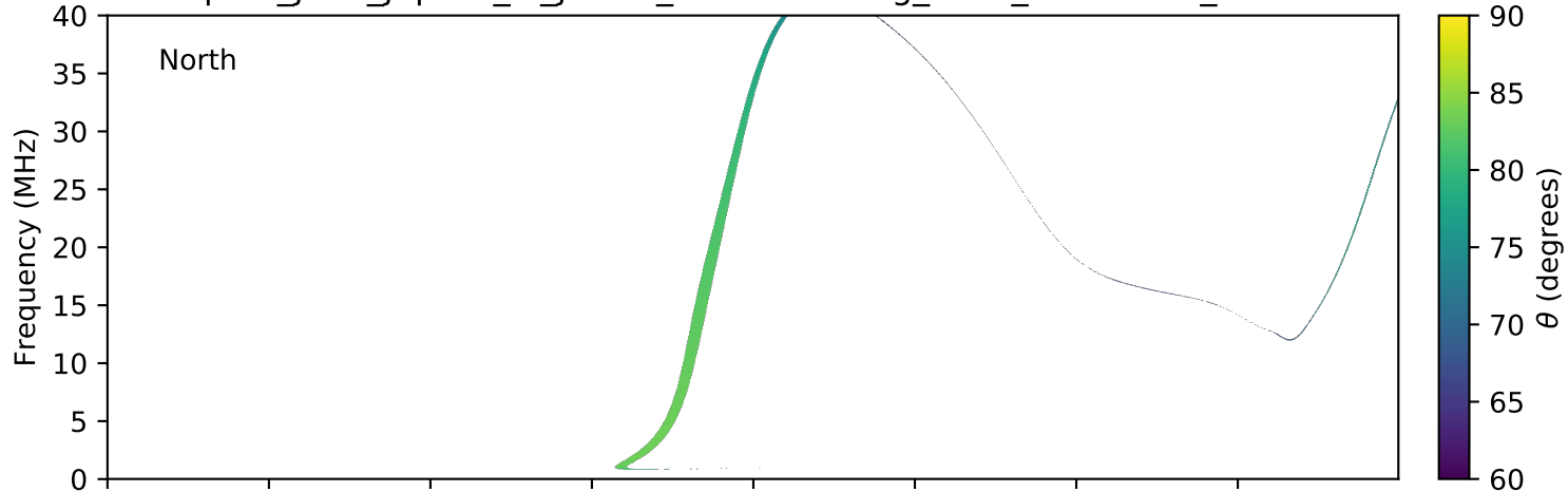
expres_juno_jupiter_io_jrm09_lossc-wid1deg_3kev_20170114_v01.cdf
