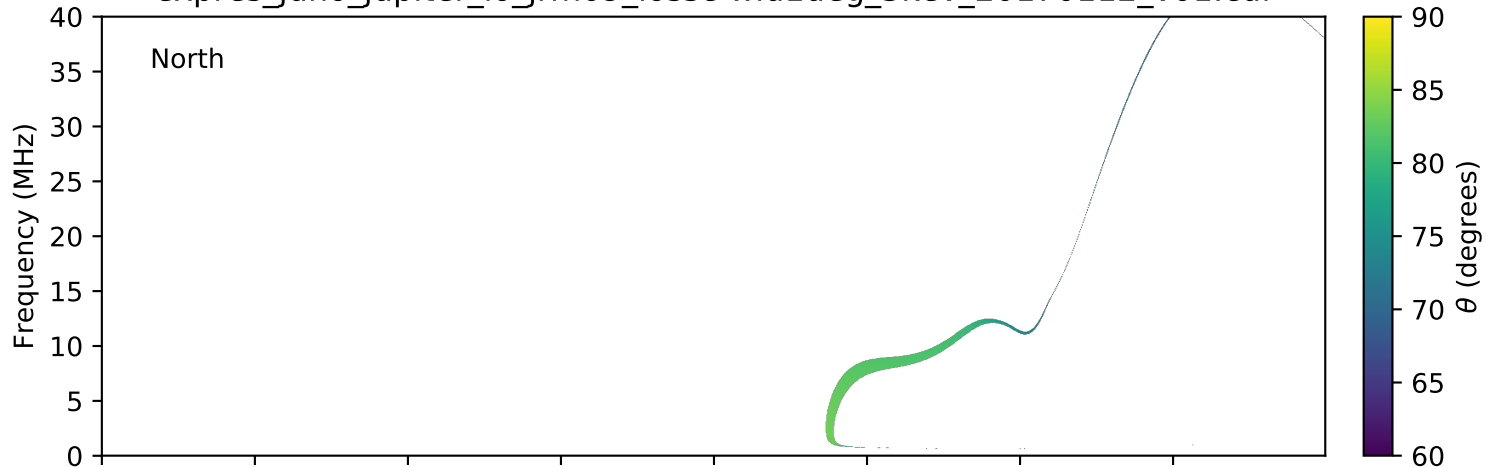
expres_juno_jupiter_io_jrm09_lossc-wid1deg_3kev_20170112_v01.cdf
