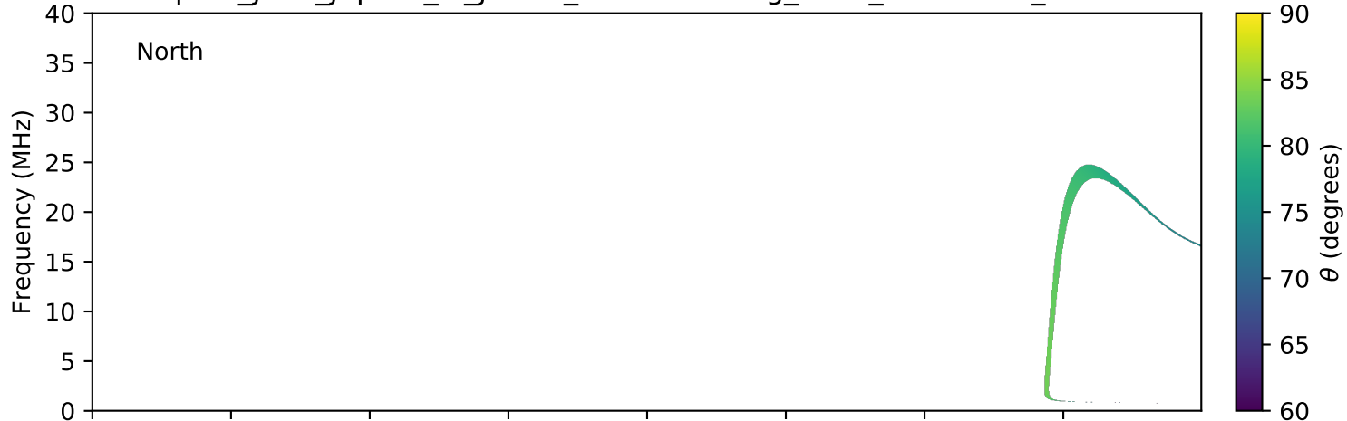
expres_juno_jupiter_io_jrm09_lossc-wid1deg_3kev_20170110_v01.cdf
