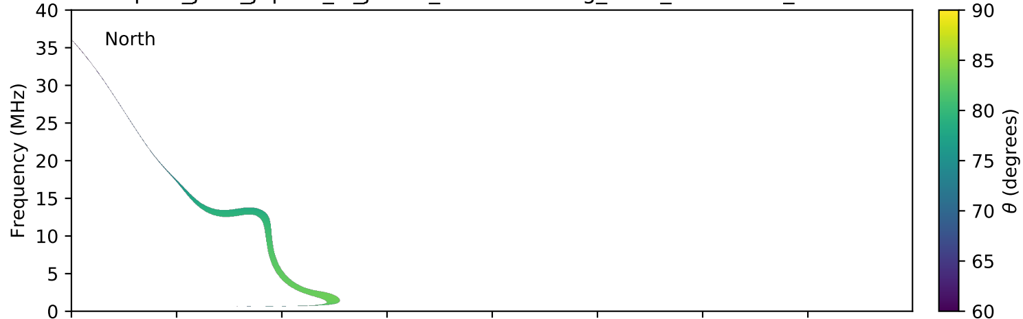
expres_juno_jupiter_io_jrm09_lossc-wid1deg_3kev_20170106_v01.cdf
