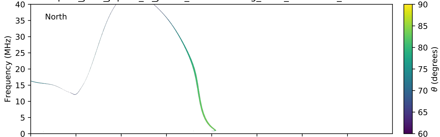
expres_juno_jupiter_io_jrm09_lossc-wid1deg_3kev_20170104_v01.cdf
