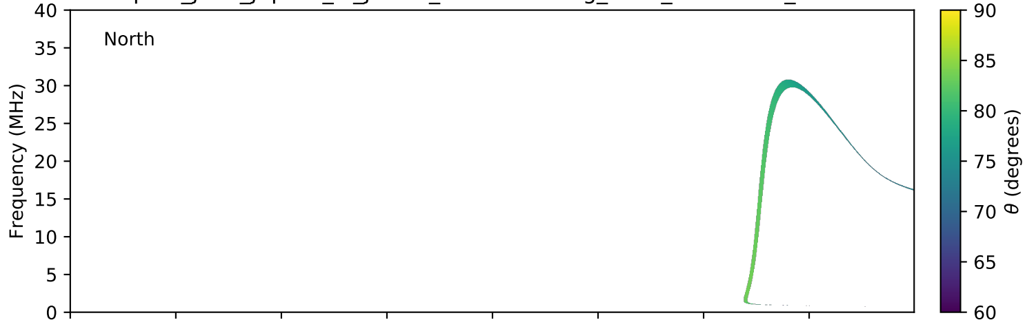
expres_juno_jupiter_io_jrm09_lossc-wid1deg_3kev_20170103_v01.cdf
