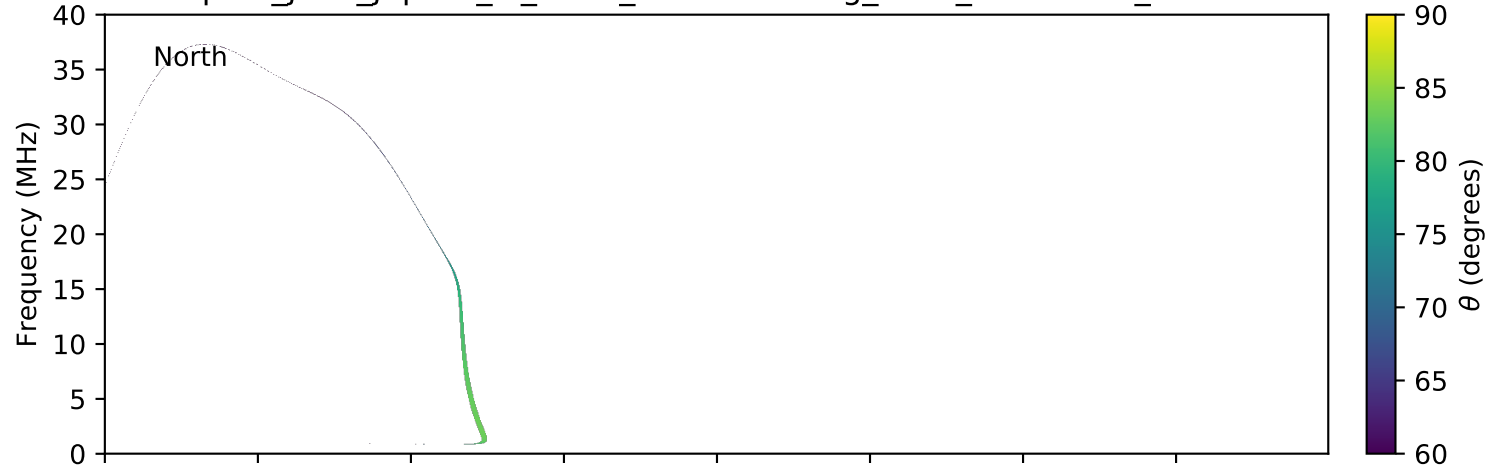
expres_juno_jupiter_io_isaac_lossc-wid1deg_3kev_20170129_v01.cdf
