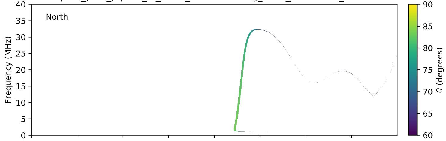
expres_juno_jupiter_io_isaac_lossc-wid1deg_3kev_20170128_v01.cdf
