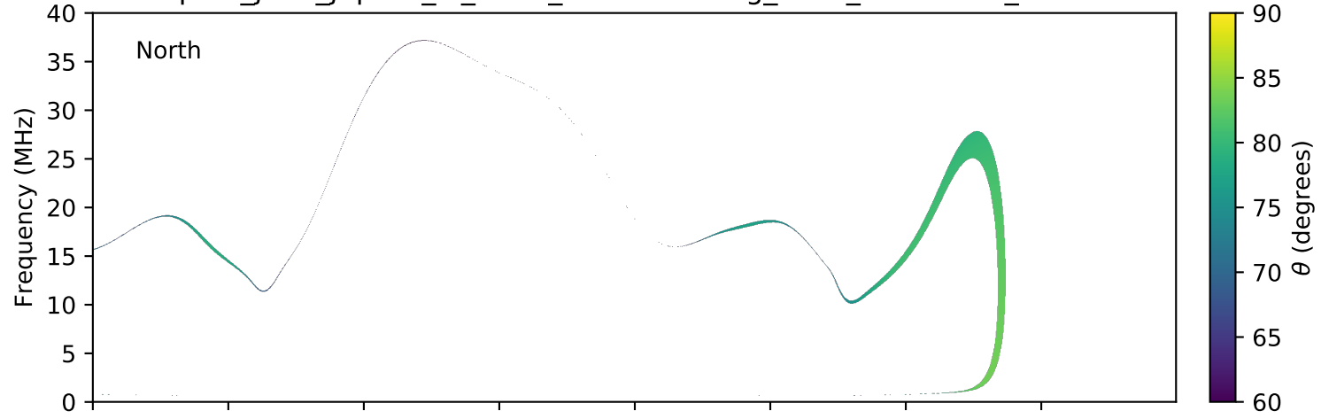
expres_juno_jupiter_io_isaac_lossc-wid1deg_3kev_20170125_v01.cdf
