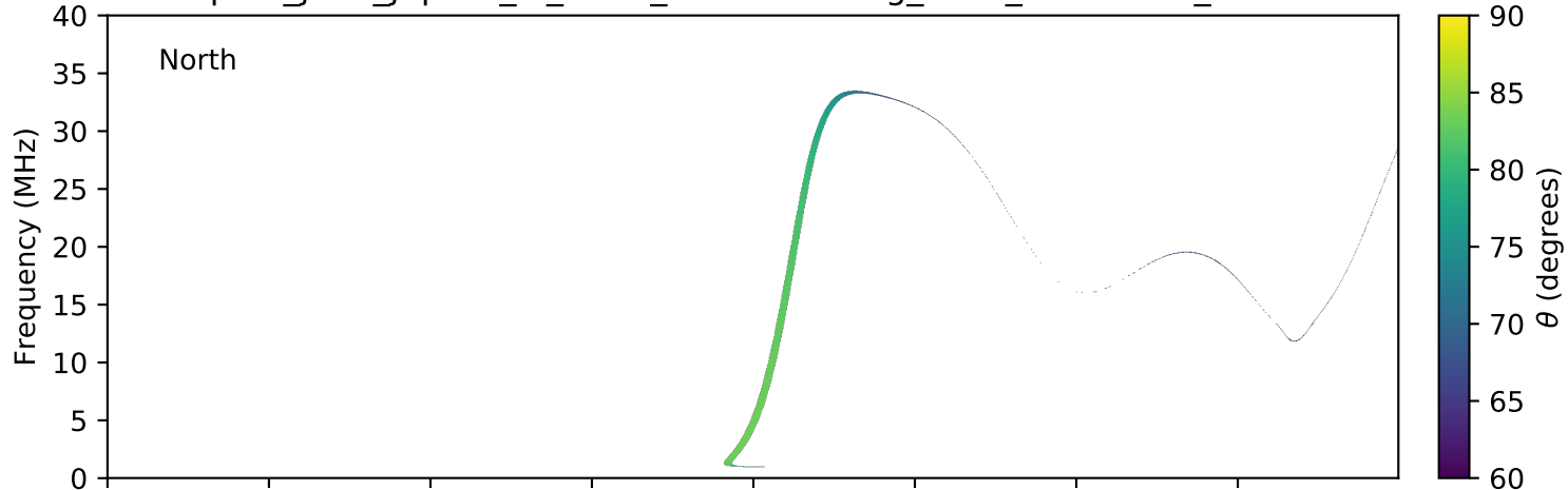
expres_juno_jupiter_io_isaac_lossc-wid1deg_3kev_20170121_v01.cdf
