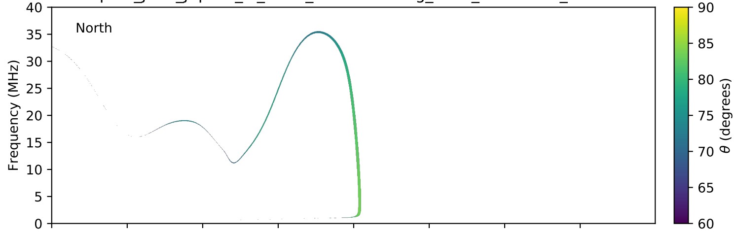
expres_juno_jupiter_io_isaac_lossc-wid1deg_3kev_20170120_v01.cdf
