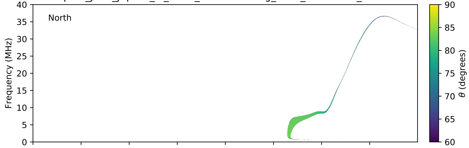
expres_juno_jupiter_io_isaac_lossc-wid1deg_3kev_20170119_v01.cdf
