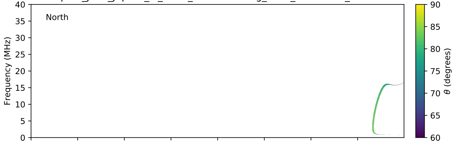
expres_juno_jupiter_io_isaac_lossc-wid1deg_3kev_20170117_v01.cdf
