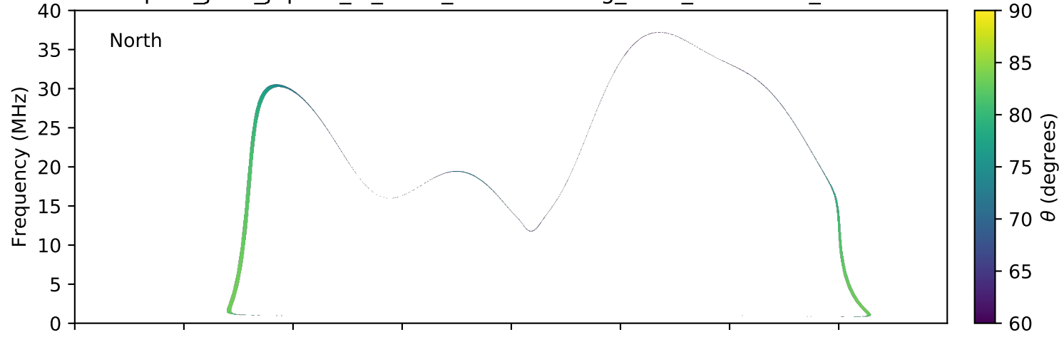
expres_juno_jupiter_io_isaac_lossc-wid1deg_3kev_20170116_v01.cdf
