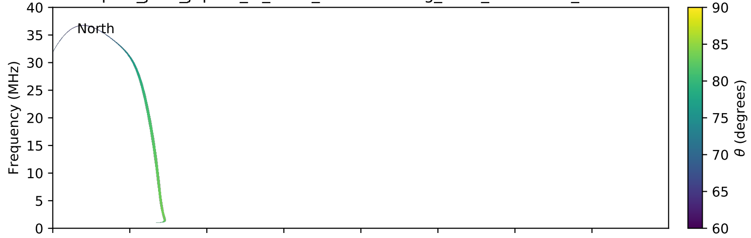
expres_juno_jupiter_io_isaac_lossc-wid1deg_3kev_20170115_v01.cdf
